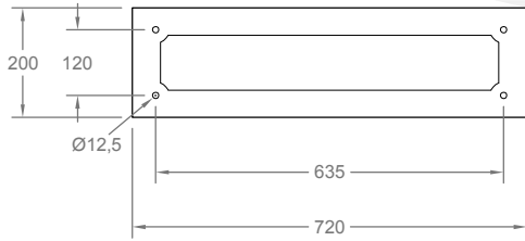
AYAK BAĞLANTI DETAYI (A-A KESİTİ) LEG CONNECTION DETAIL (SECTION A-A)
