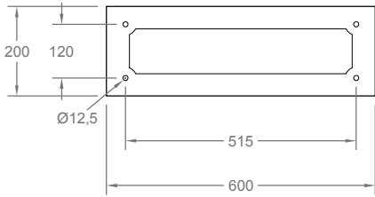
AYAK BAĞLANTI DETAYI (A-A KESİTİ) LEG CONNECTION DETAIL (SECTION A-A)
