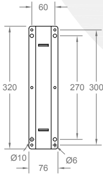
DUVAR MONTAJ PLAKASI WALL MOUNTING PLATE
